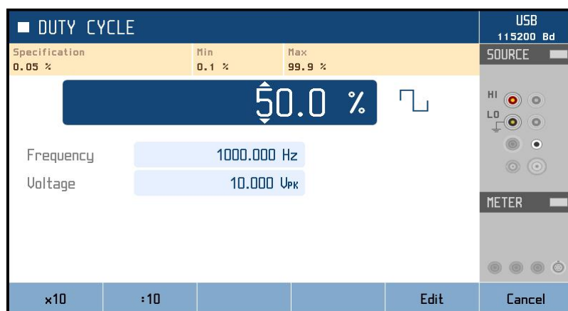
Obr. 32 Duty cycle
