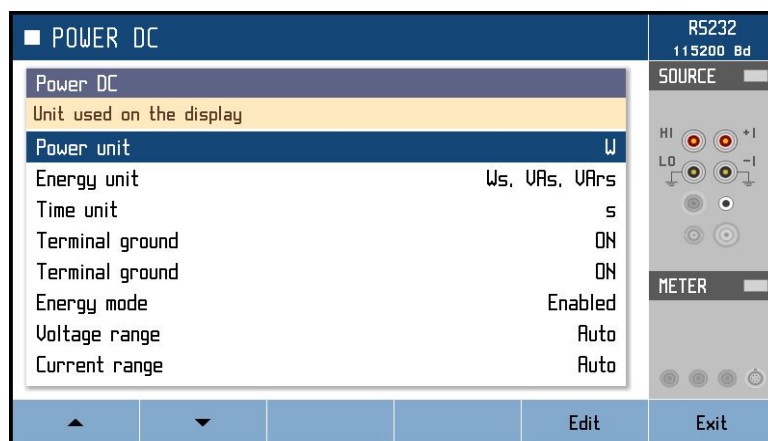
Obr. 11 Device menu
