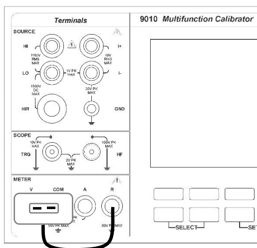
Obr. 43 Thermocouple output through 91 Adapter
