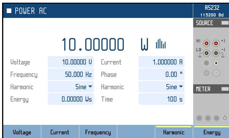
Obr. 29 Energy mode
