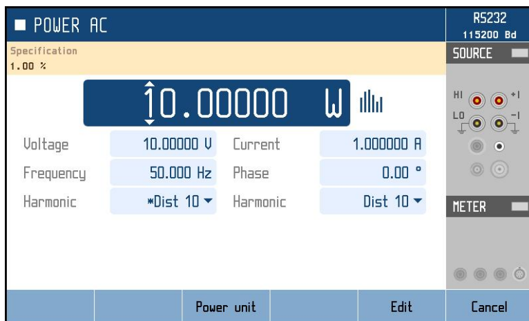
Obr. 28 Harmonic mode
