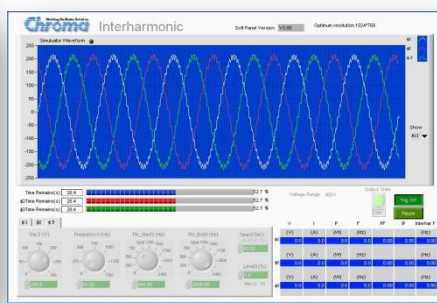
Interharmonic Test
