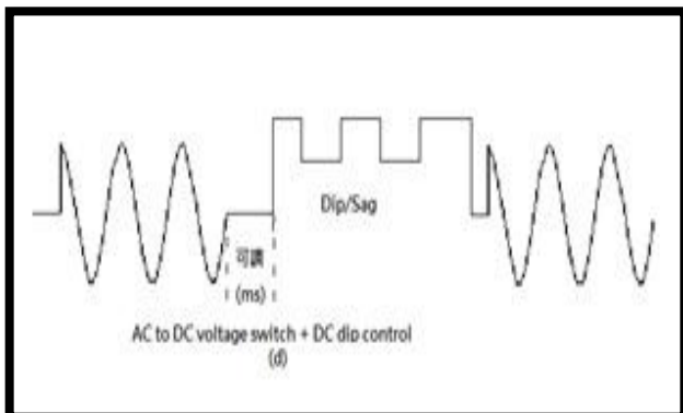
Voltage waveform test requirement
