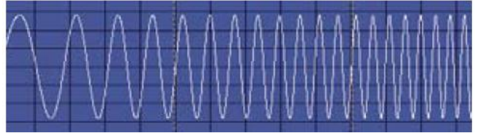
Output voltage waveform based on frequency of slew rate setting
